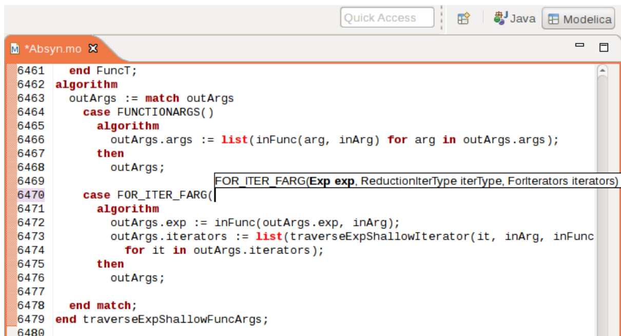
Figure 8.14: Code assistance when writing cases with records in MetaModelica.
