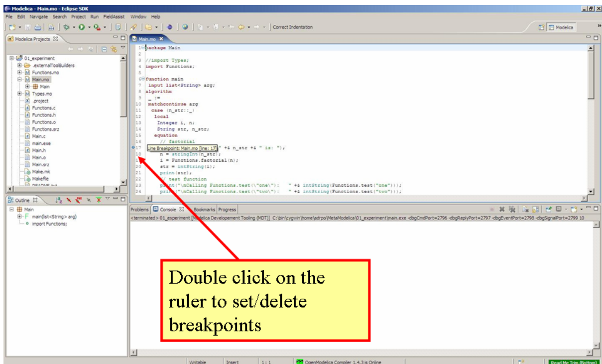
Figure 9.4: Setting/deleting breakpoints.
