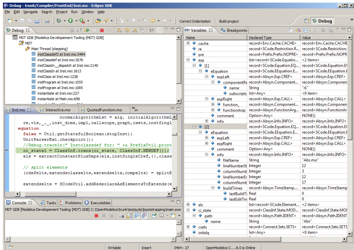
Figure 9.1: Debugging functionality.
