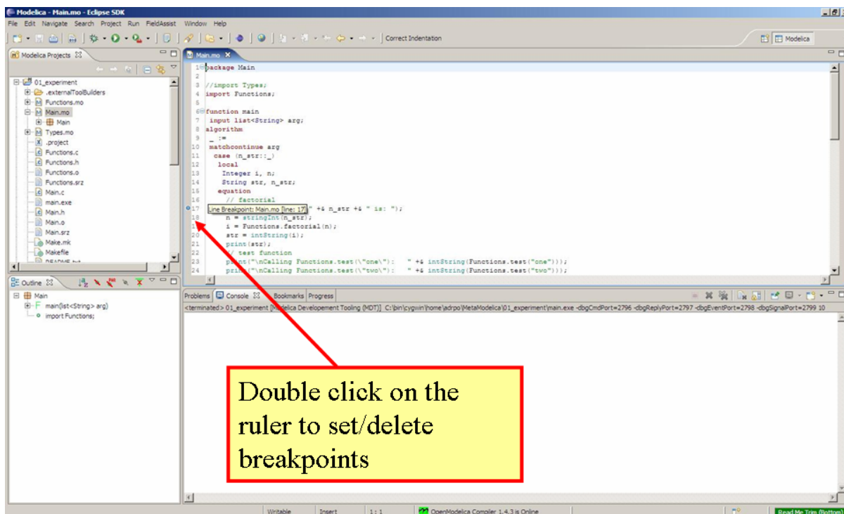
Figure 9.4: Setting/deleting breakpoints.
