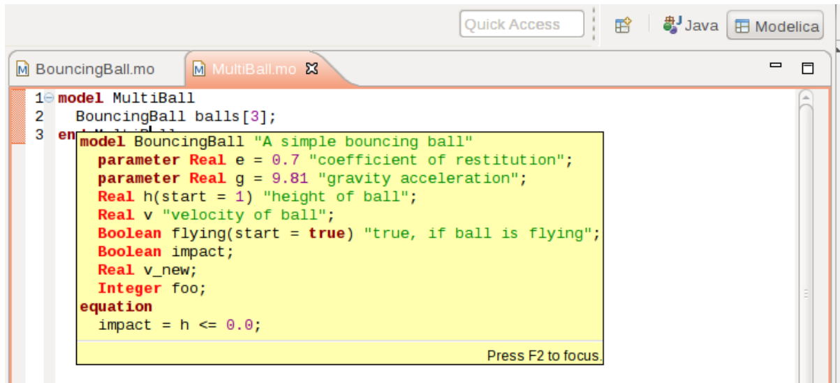
Figure 8.13: Displaying information for identifiers on hovering.
