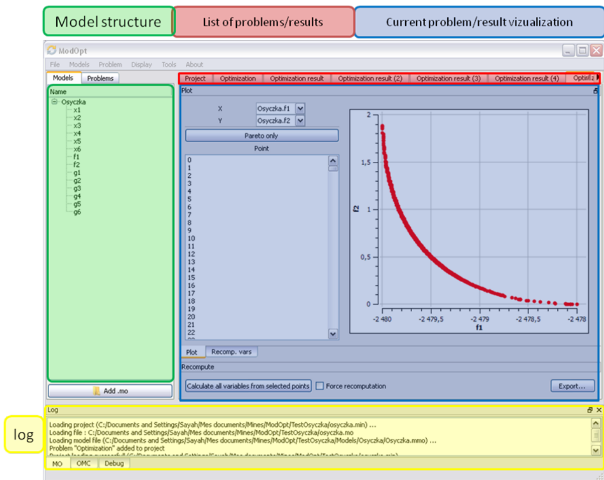
Figure 7.6: Window regions in OMOptim GUI.
