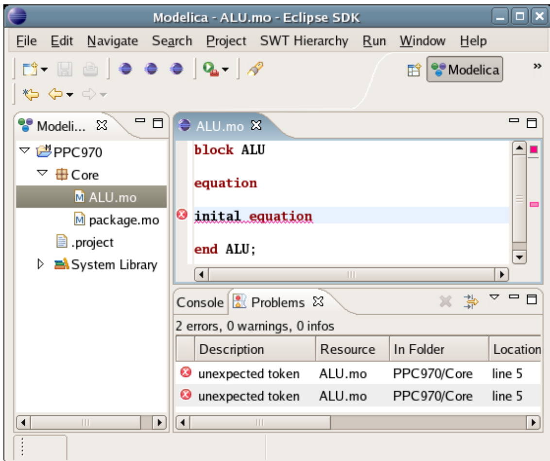
Figure 8.10: Syntax checking.
