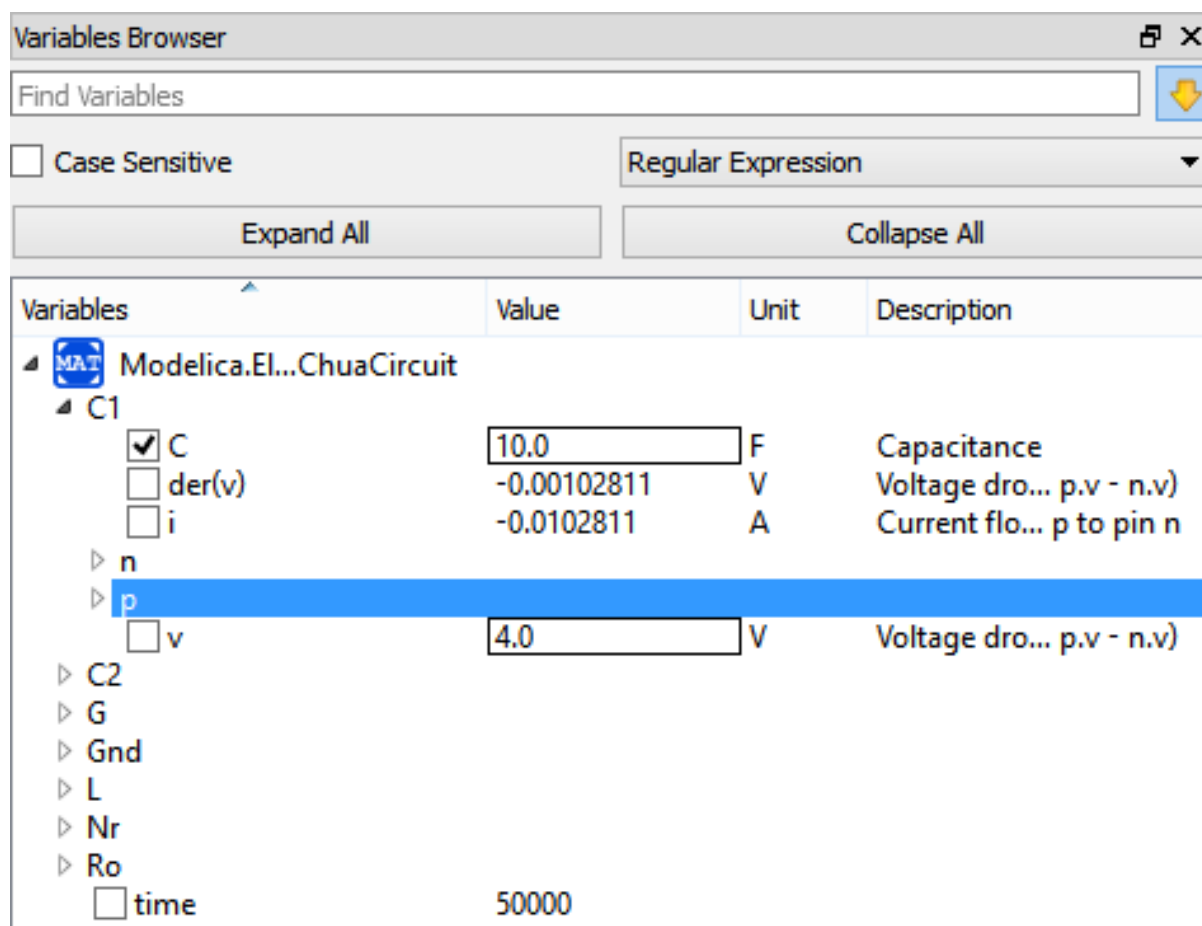
Figure 2.5: Variables Browser.
