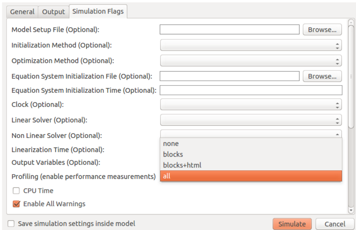
Figure 10.1: Setting up the profiler from OMEdit.
