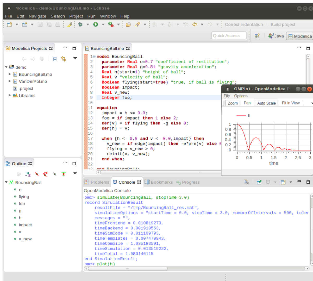
Figure 8.16: Simulation from MDT Console.
