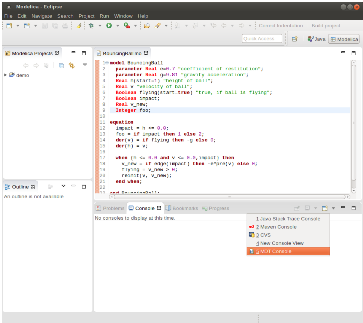
Figure 8.15: Activate the MDT Console.
