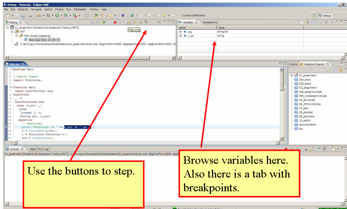
Figure 9.7: The debugging perspective.
