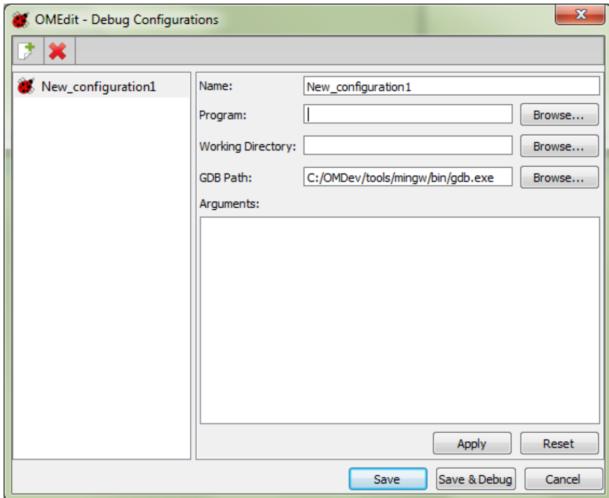
Figure 4.4: Debug Configurations.
