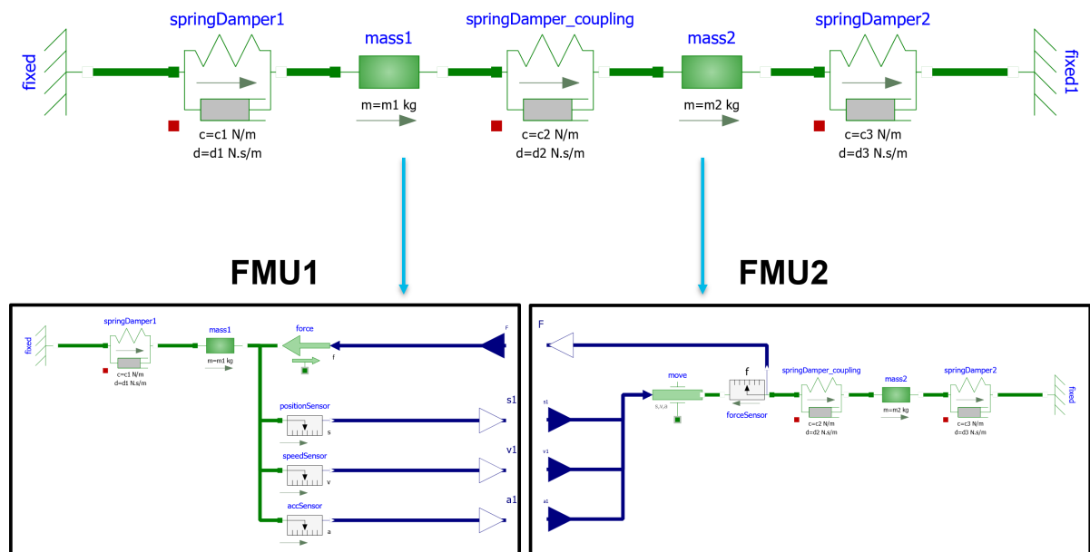
Figure 13.11: Dual mass oscillator Modelica model (diagram view) and FMUs
