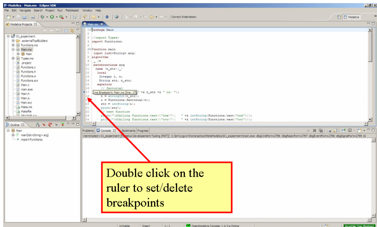
Figure 20.4: Setting/deleting breakpoints.
