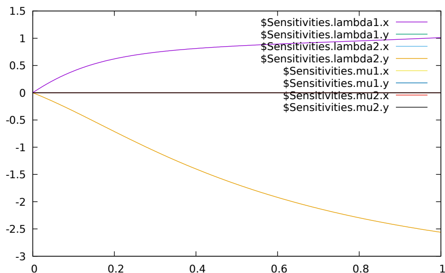
Figure 12.1: Results of the sensitivities calculated by IDA solver.
