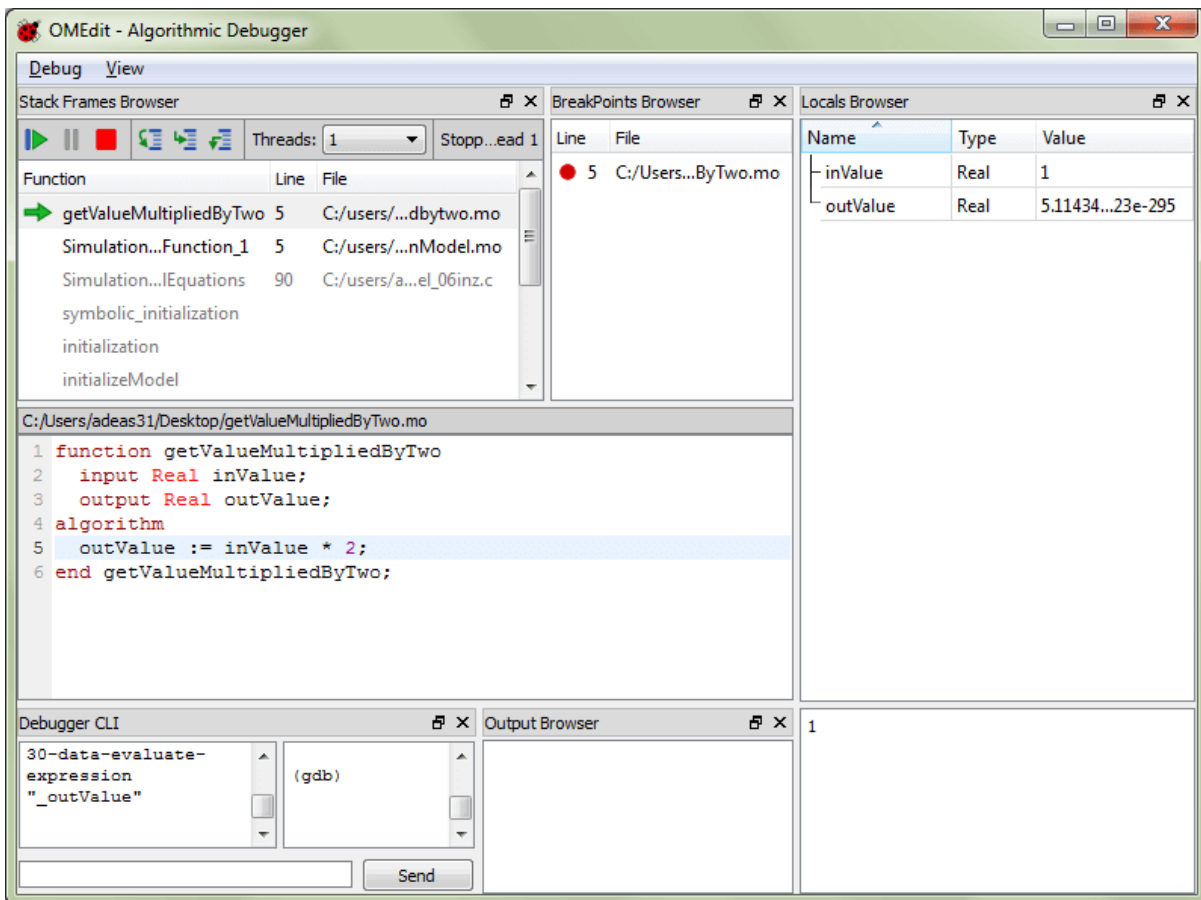
Figure 4.6: Algorithmic Debugger.
