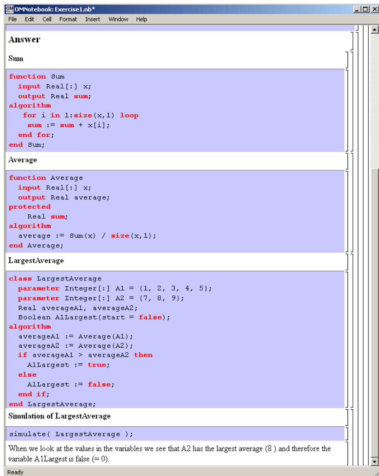
Figure 6.6: The answer section to Exercise 1 in Chapter 9 of DrModelica.
