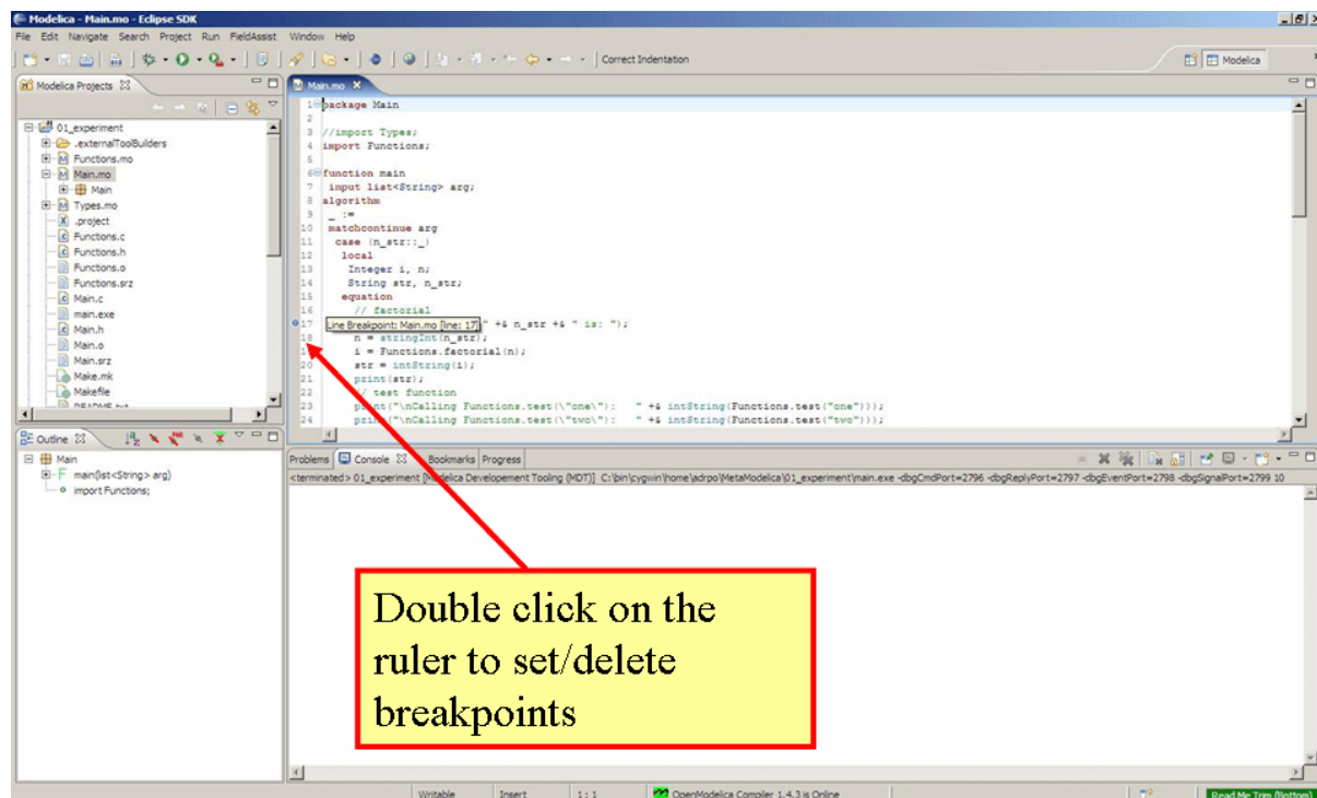
Figure 18.4: Setting/deleting breakpoints.
