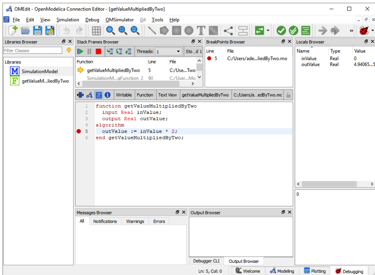
Figure 6.6: Algorithmic Debugger.
