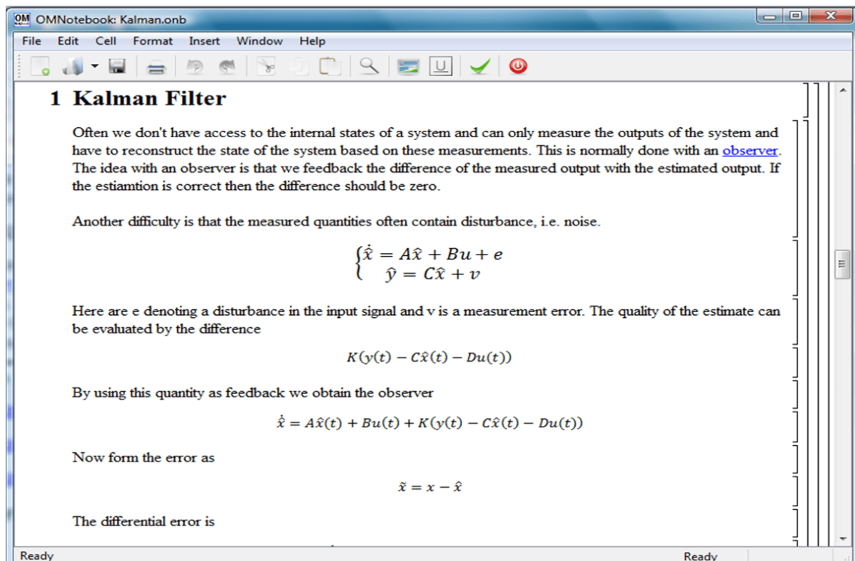
Figure 11.12: Theory background about Kalman filter.
