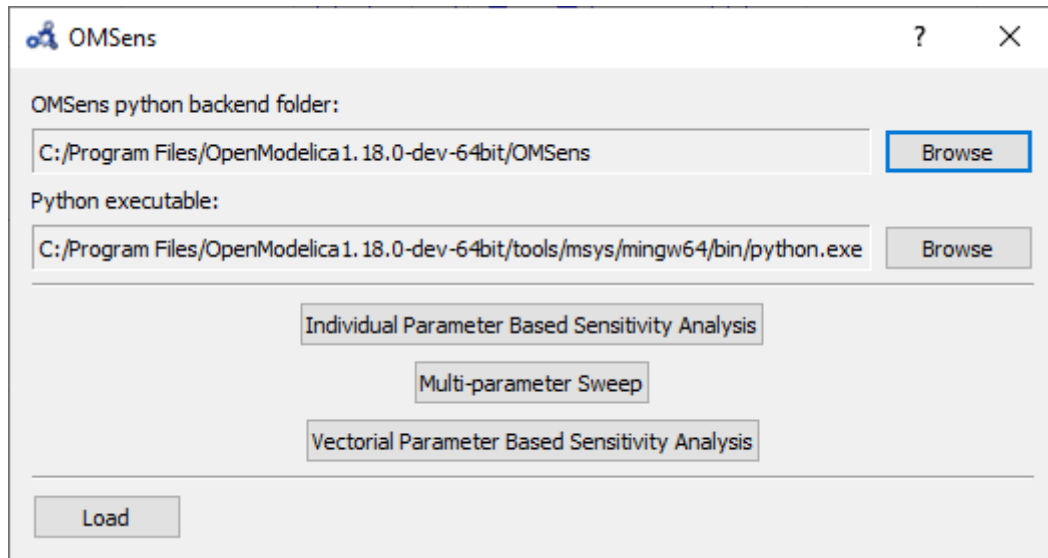
Figure 19.3: OMSens window.
