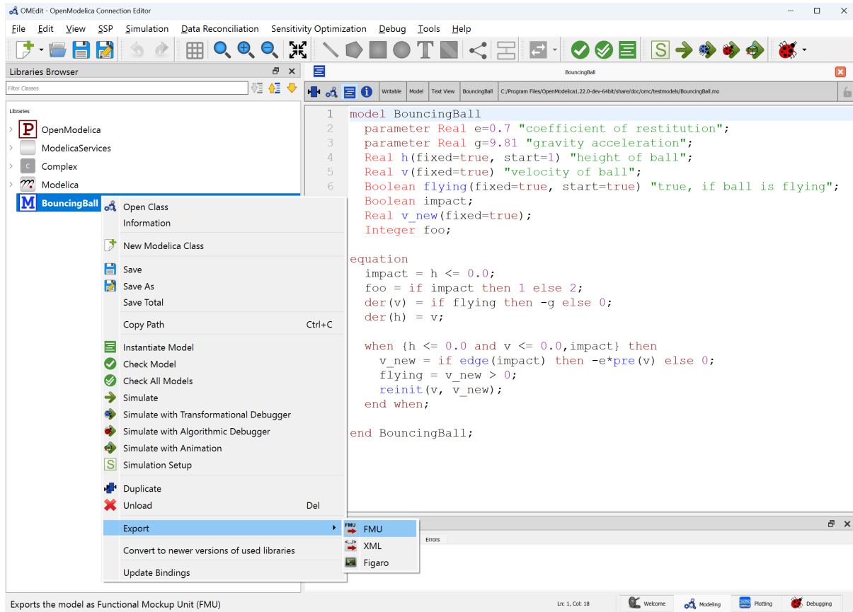
Figure 13.1: FMI Export.
