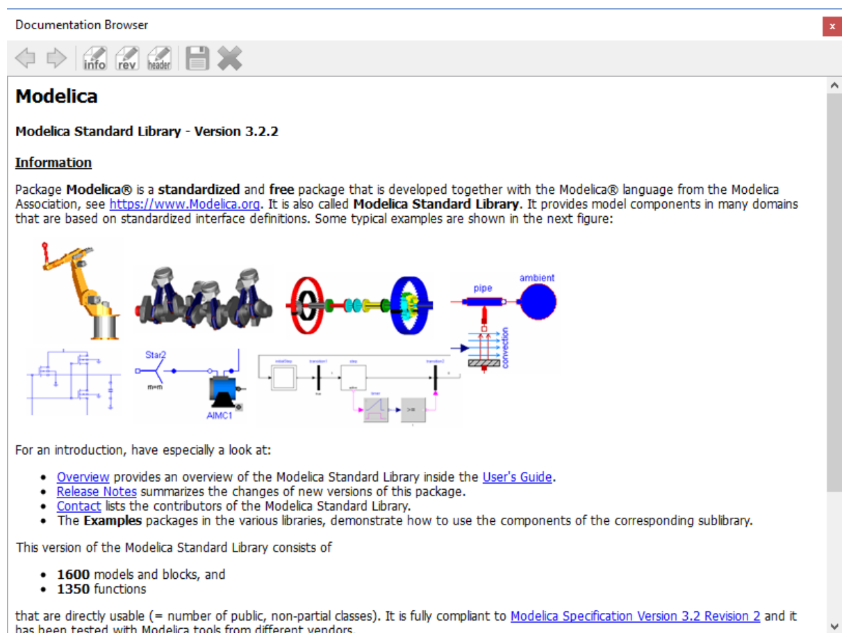
Figure 3.3: Documentation Browser.
