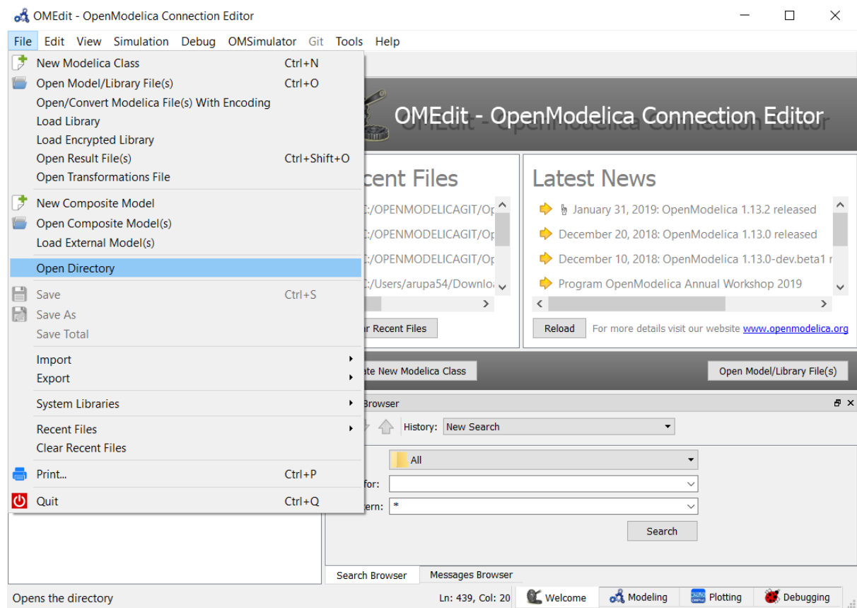
Figure 3.18: open-directory
