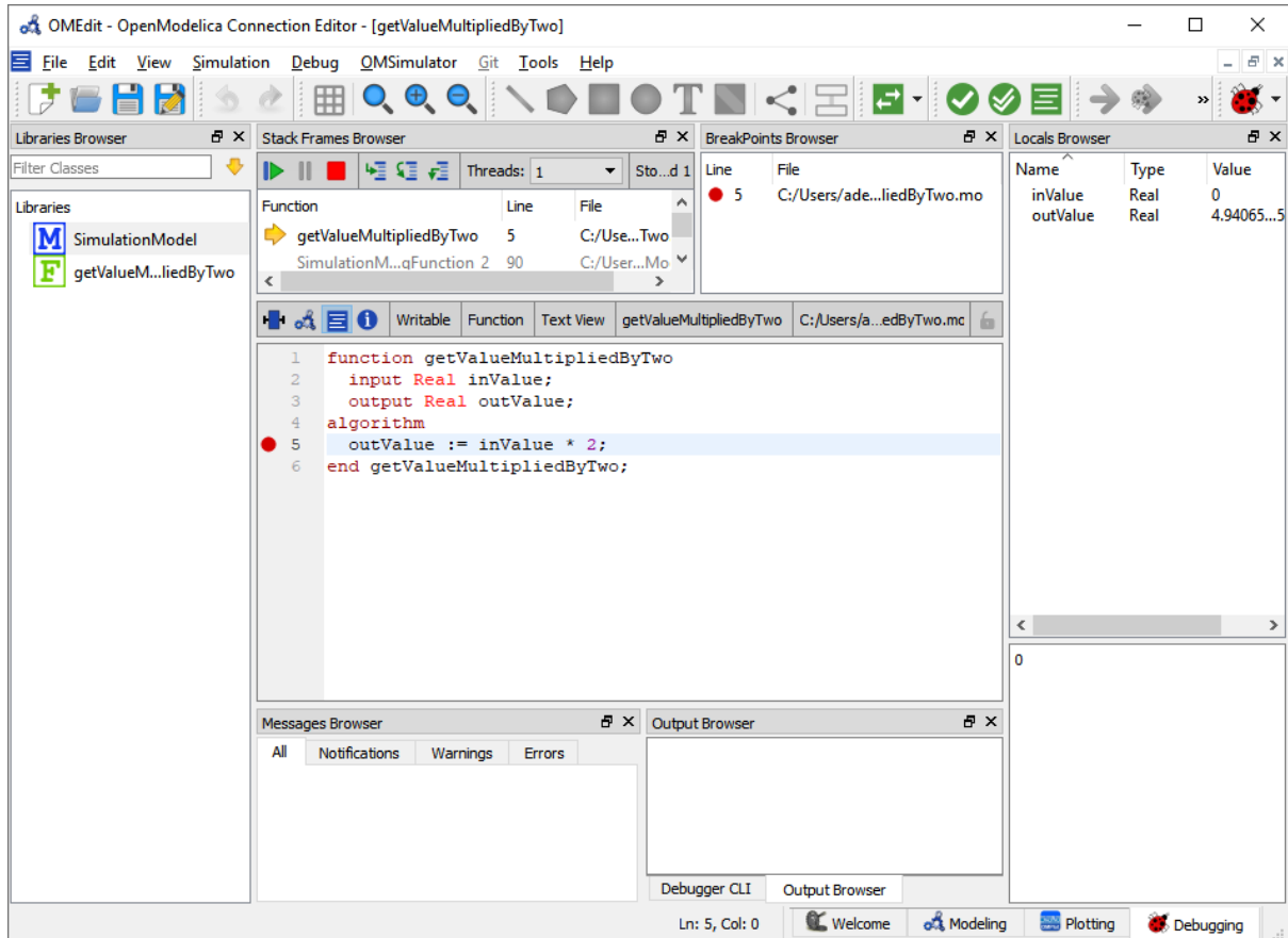
Figure 7.6: Algorithmic Debugger.
