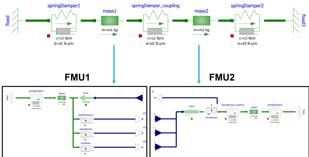
Fig. 10: Dual mass oscillator Modelica model (diagram view) and FMUs
